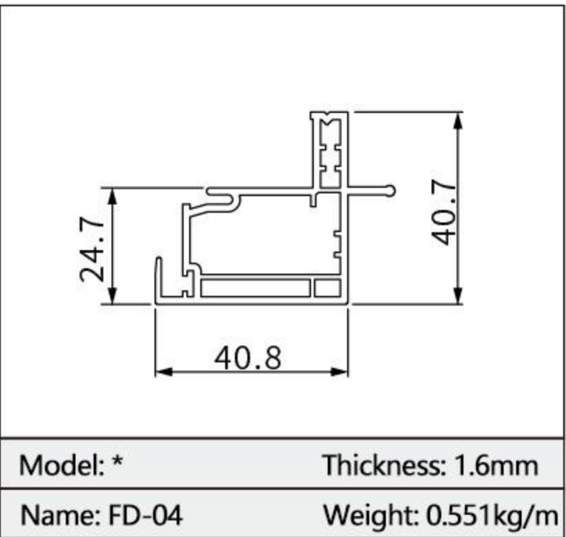
HUNG WINDOW
