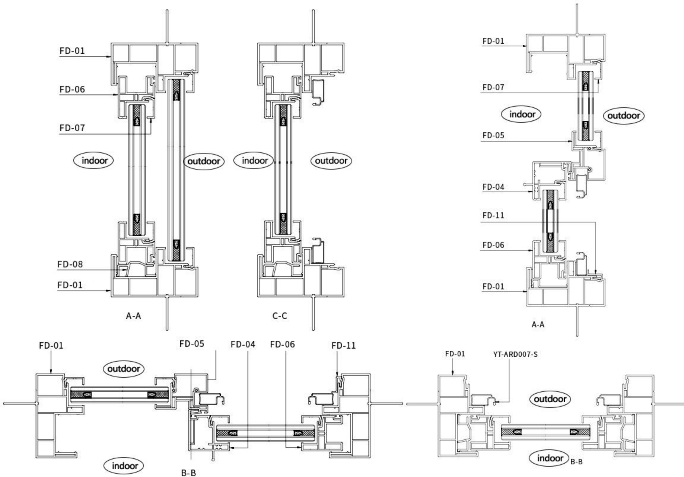
SLIDING WINDOW
